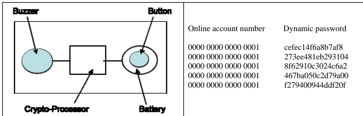
Figure 2. Calculation of dynamic passwords by the chip
